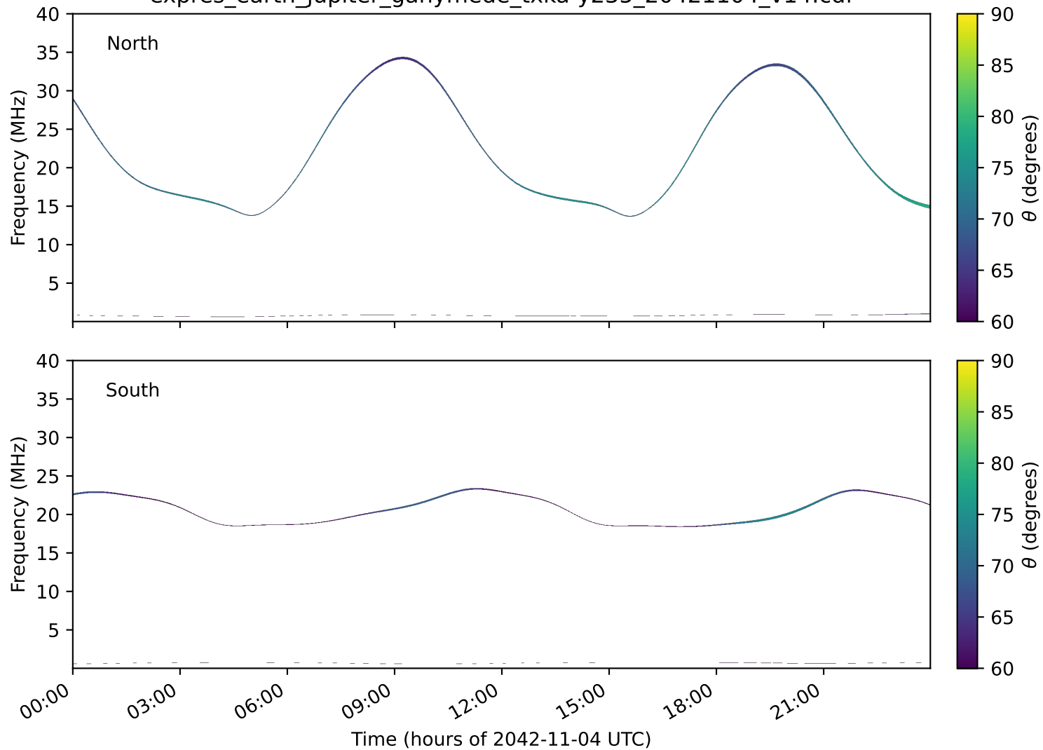
expres_earth_jupiter_ganymede_txka-y235_20421104_v14.cdf
