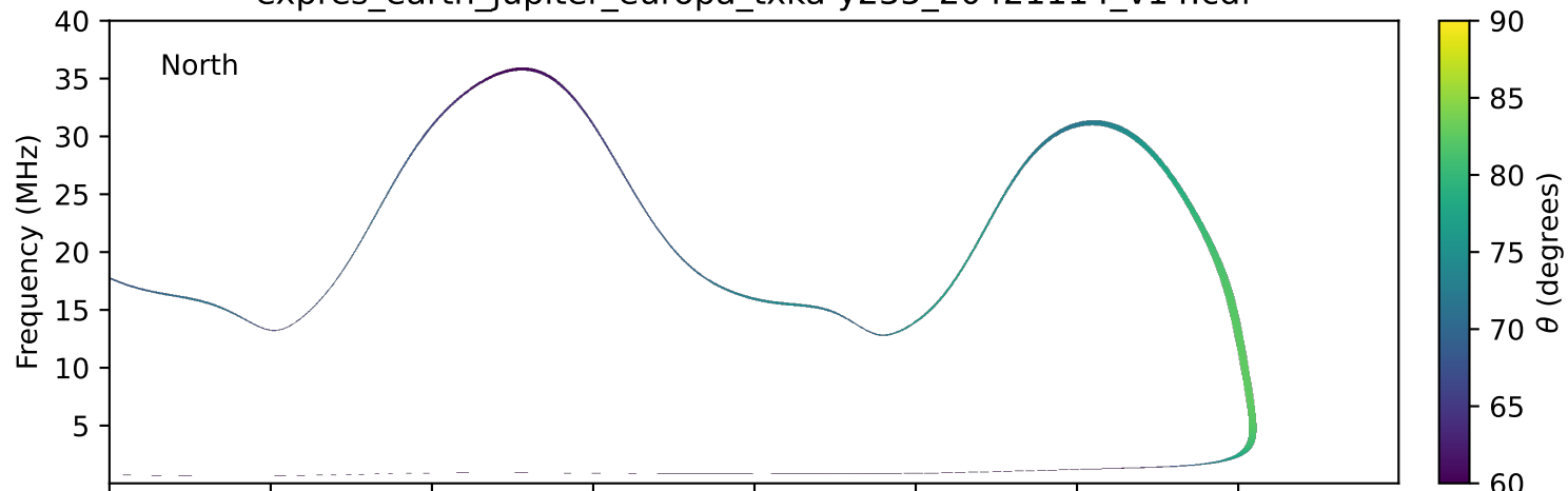
expres_earth_jupiter_europa_txka-y235_20421114_v14.cdf
