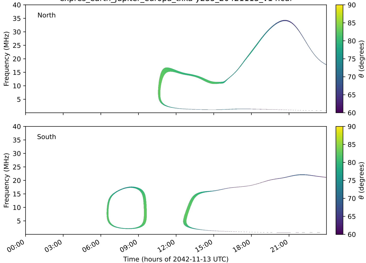
expres_earth_jupiter_europa_txka-y235_20421113_v14.cdf
