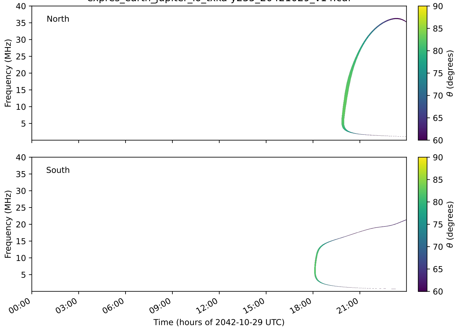
expres_earth_jupiter_io_txka-y235_20421029_v14.cdf
