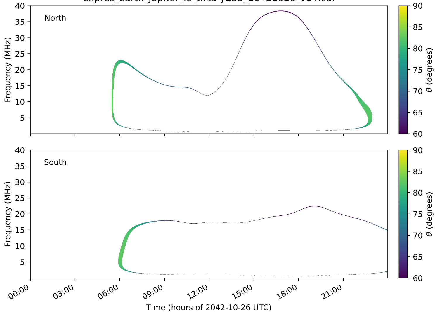
expres_earth_jupiter_io_txka-y235_20421026_v14.cdf
