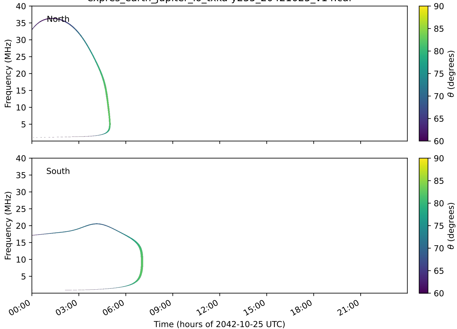
expres_earth_jupiter_io_txka-y235_20421025_v14.cdf
