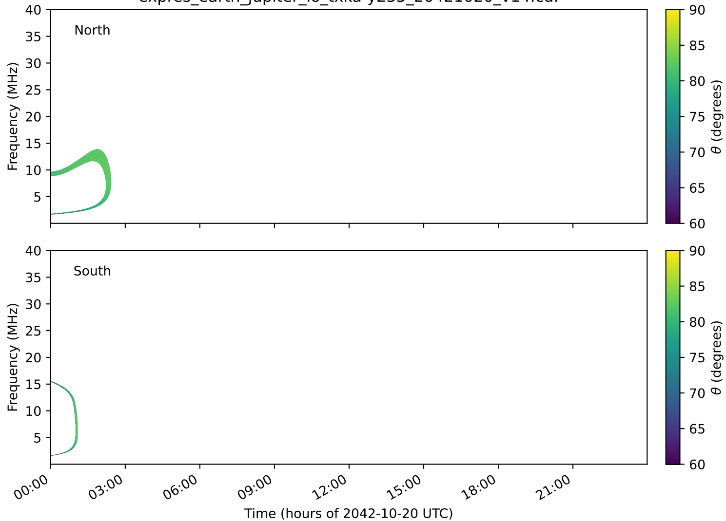
expres_earth_jupiter_io_txka-y235_20421020_v14.cdf
