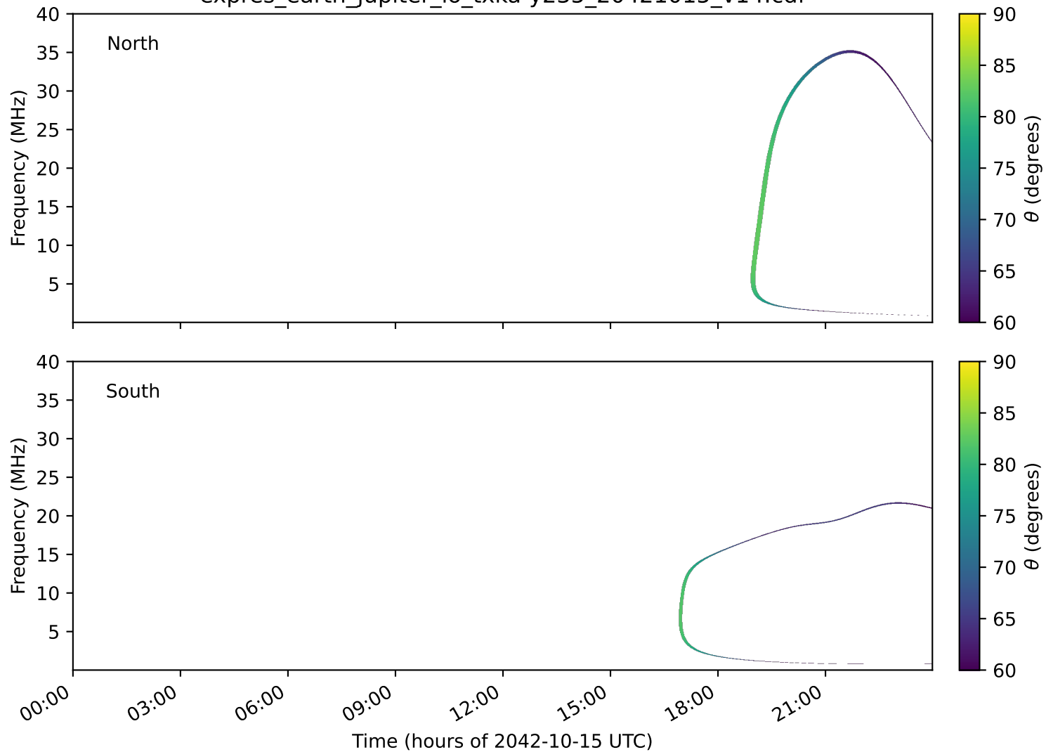
expres_earth_jupiter_io_txka-y235_20421015_v14.cdf
