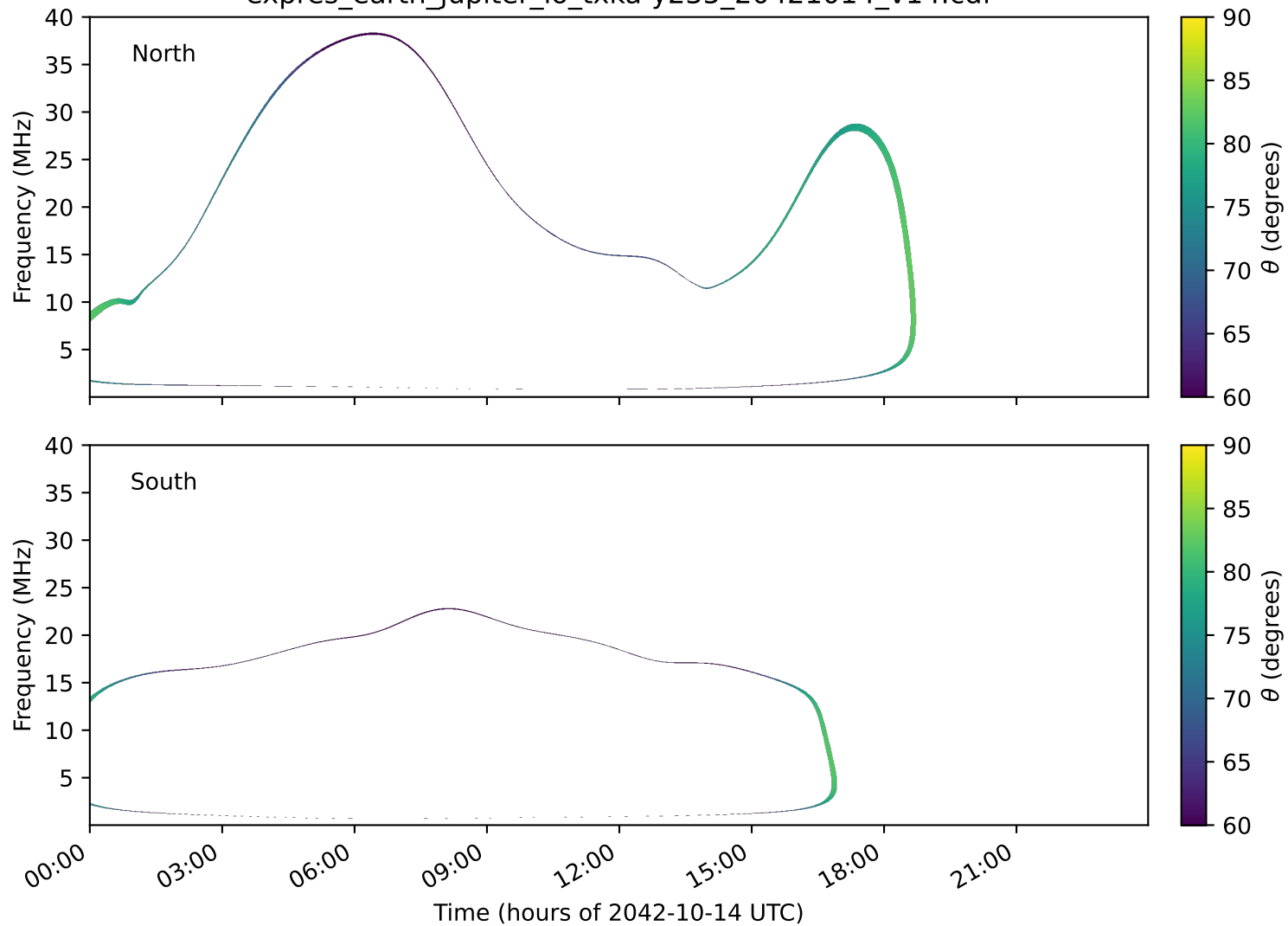
expres_earth_jupiter_io_txka-y235_20421014_v14.cdf
