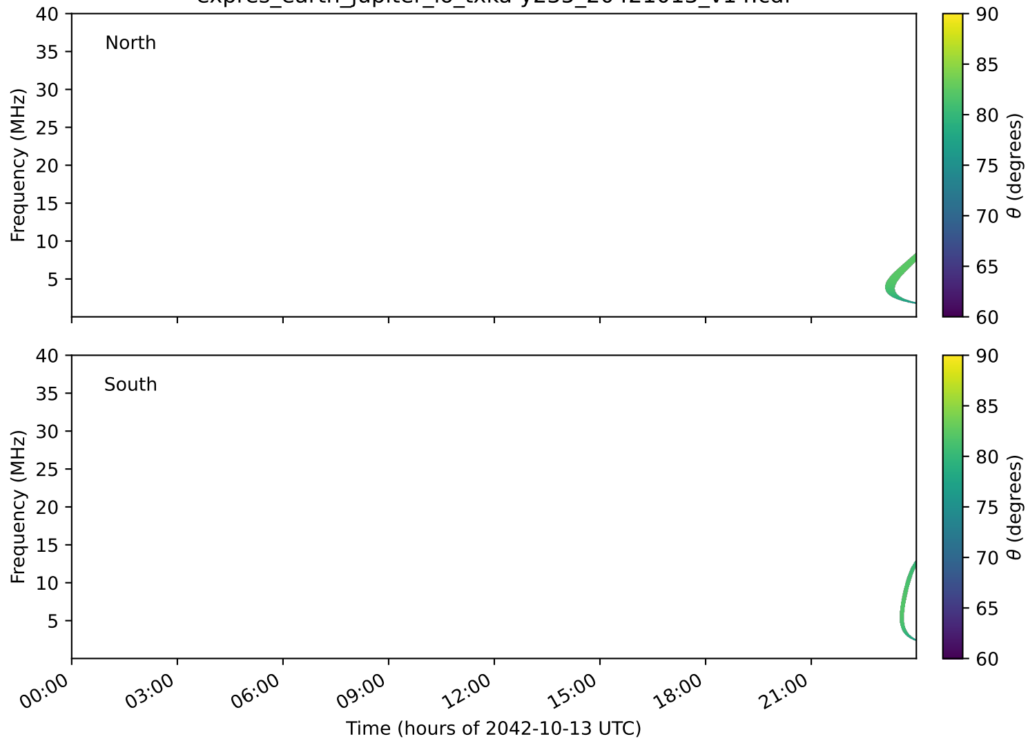
expres_earth_jupiter_io_txka-y235_20421013_v14.cdf
