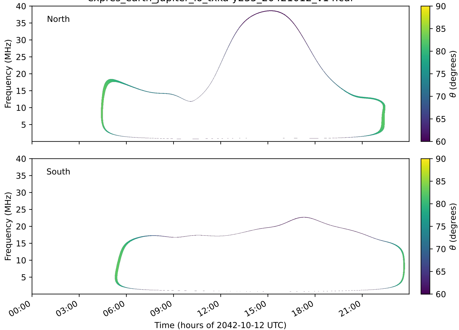
expres_earth_jupiter_io_txka-y235_20421012_v14.cdf
