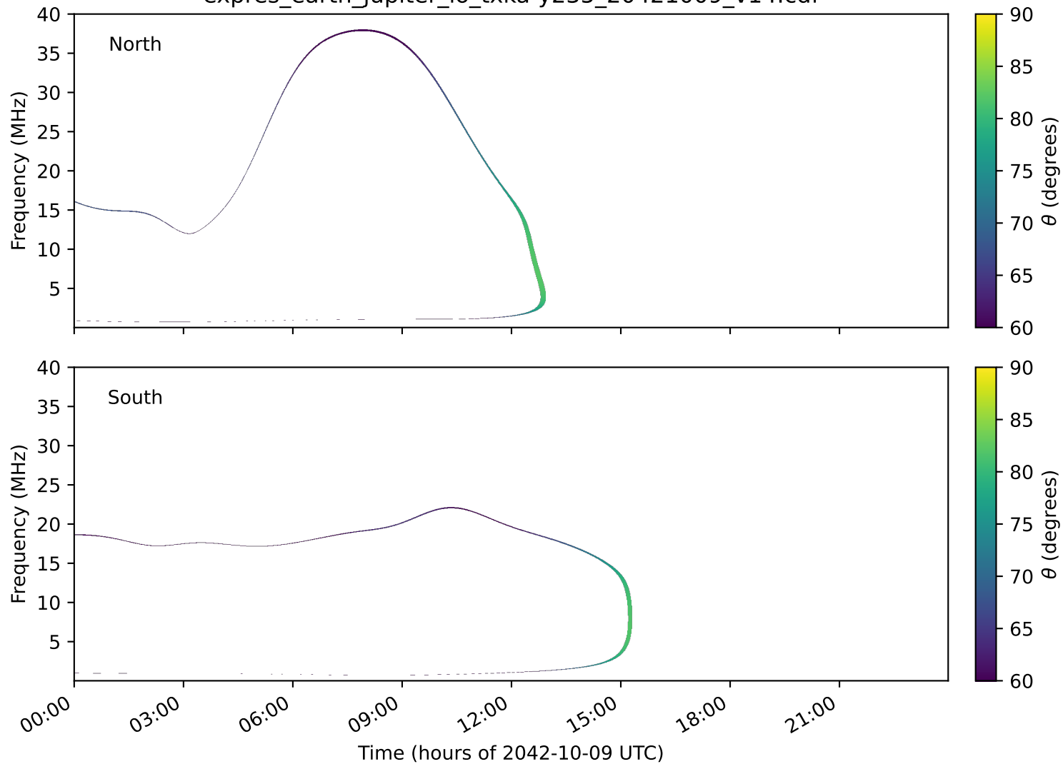
expres_earth_jupiter_io_txka-y235_20421009_v14.cdf
