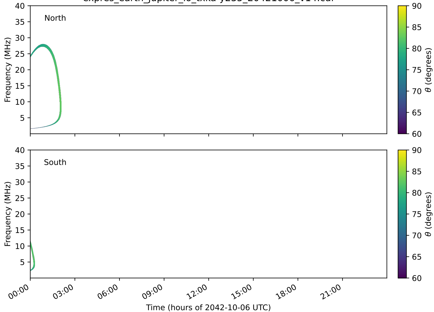
expres_earth_jupiter_io_txka-y235_20421006_v14.cdf
