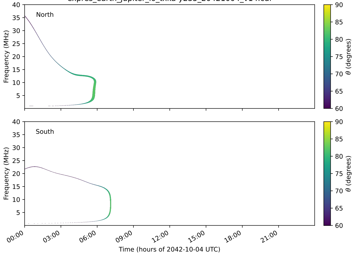
expres_earth_jupiter_io_txka-y235_20421004_v14.cdf
