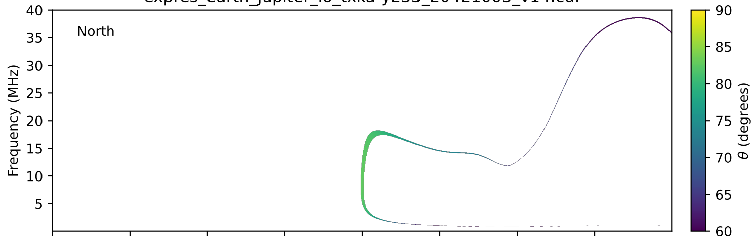
expres_earth_jupiter_io_txka-y235_20421003_v14.cdf
