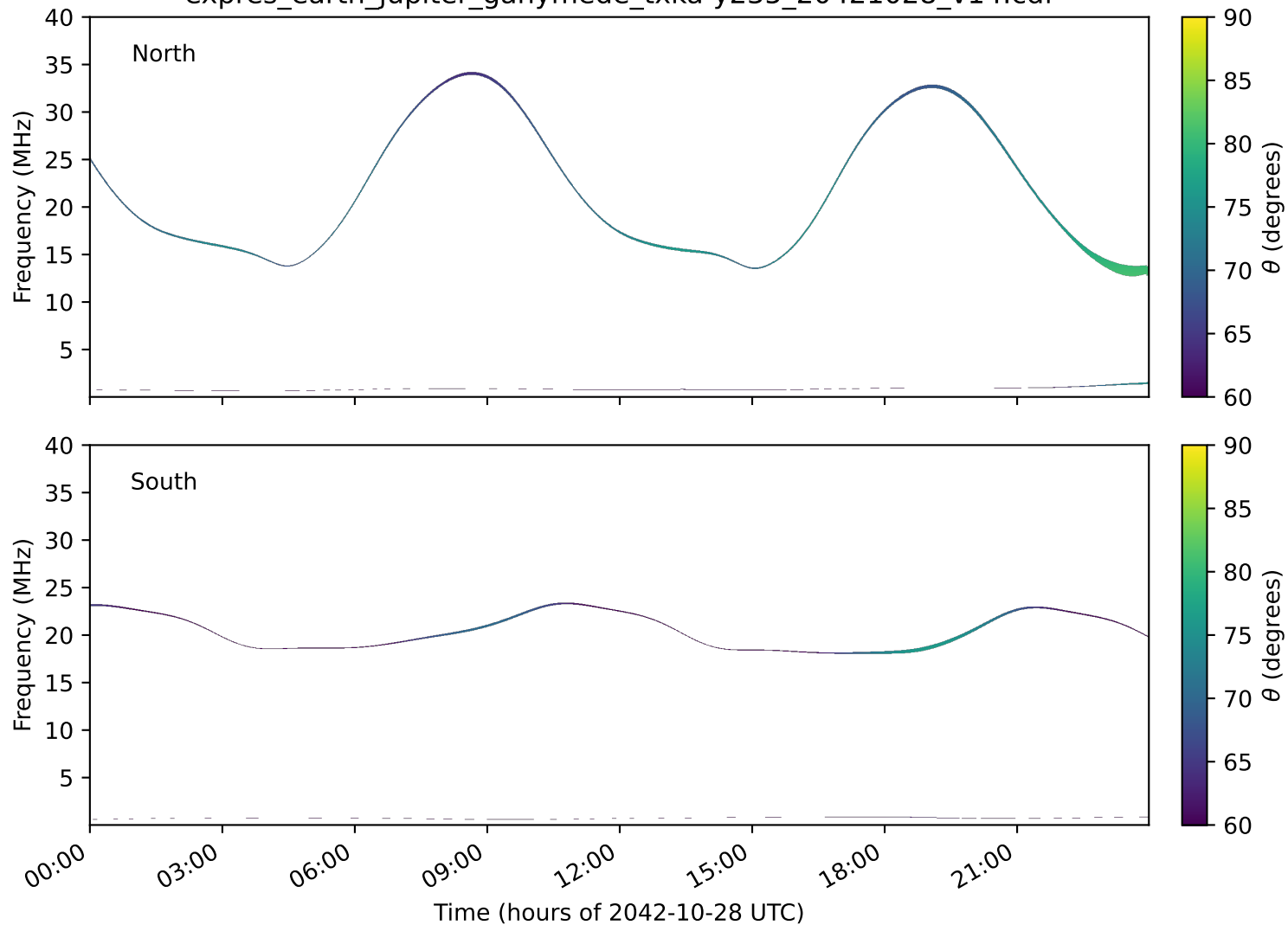
expres_earth_jupiter_ganymede_txka-y235_20421028_v14.cdf
