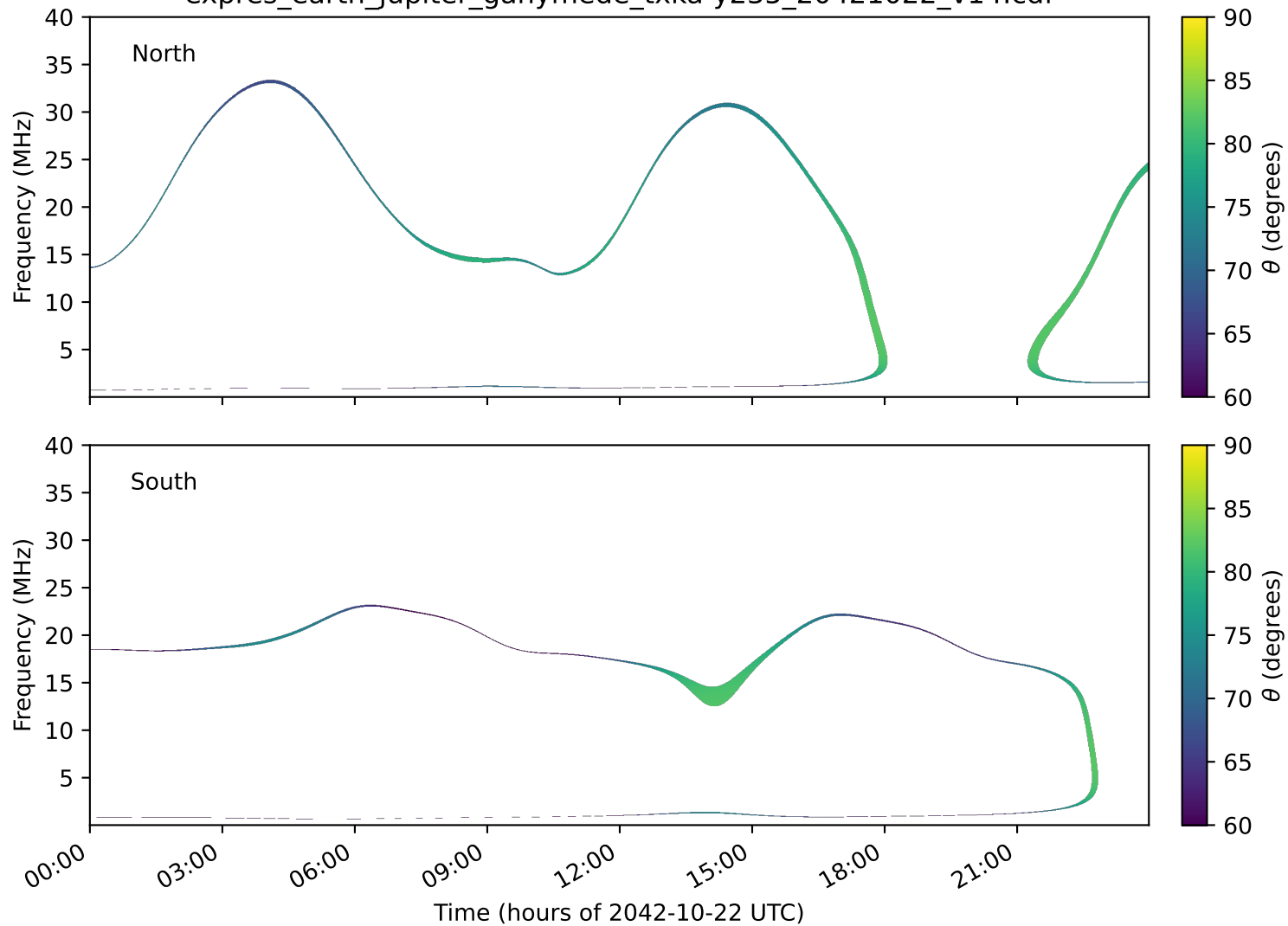
expres_earth_jupiter_ganymede_txka-y235_20421022_v14.cdf
