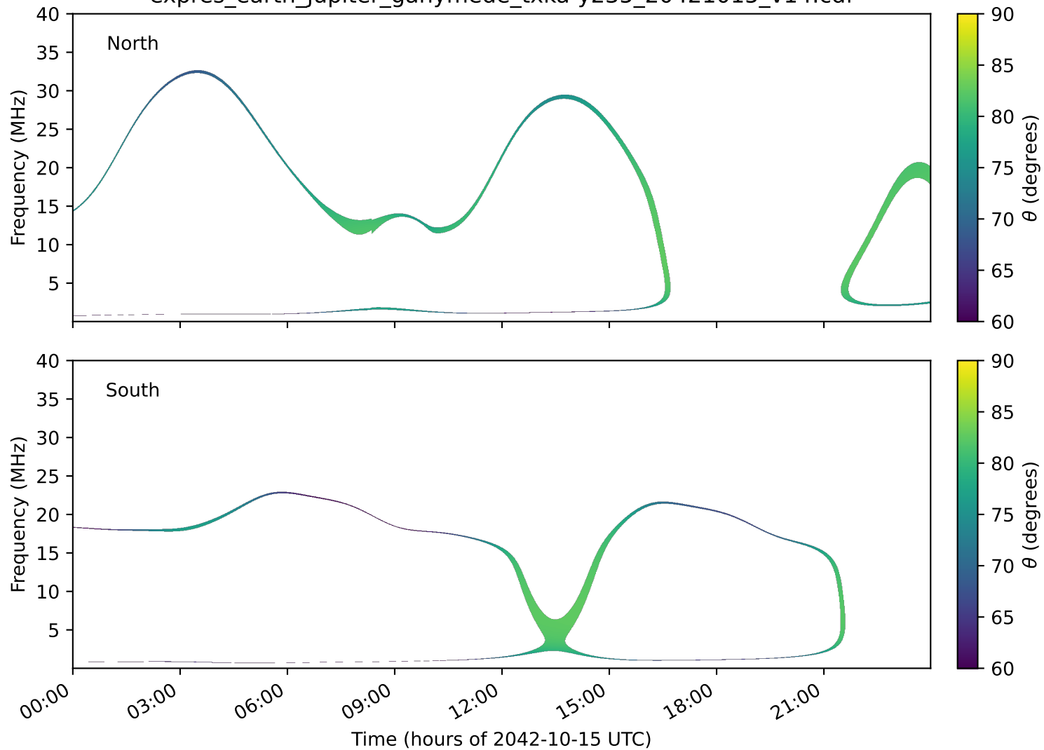
expres_earth_jupiter_ganymede_txka-y235_20421015_v14.cdf
