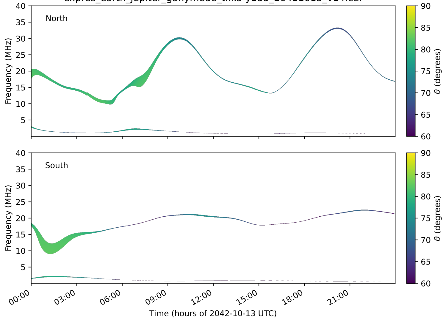
expres_earth_jupiter_ganymede_txka-y235_20421013_v14.cdf
