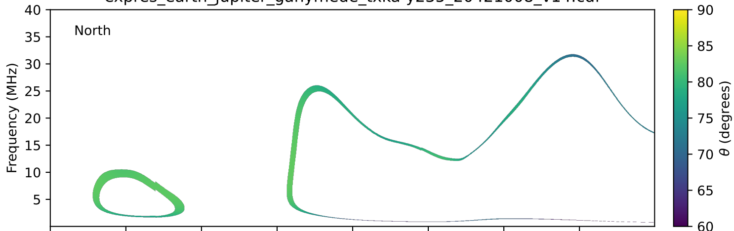
expres_earth_jupiter_ganymede_txka-y235_20421008_v14.cdf
