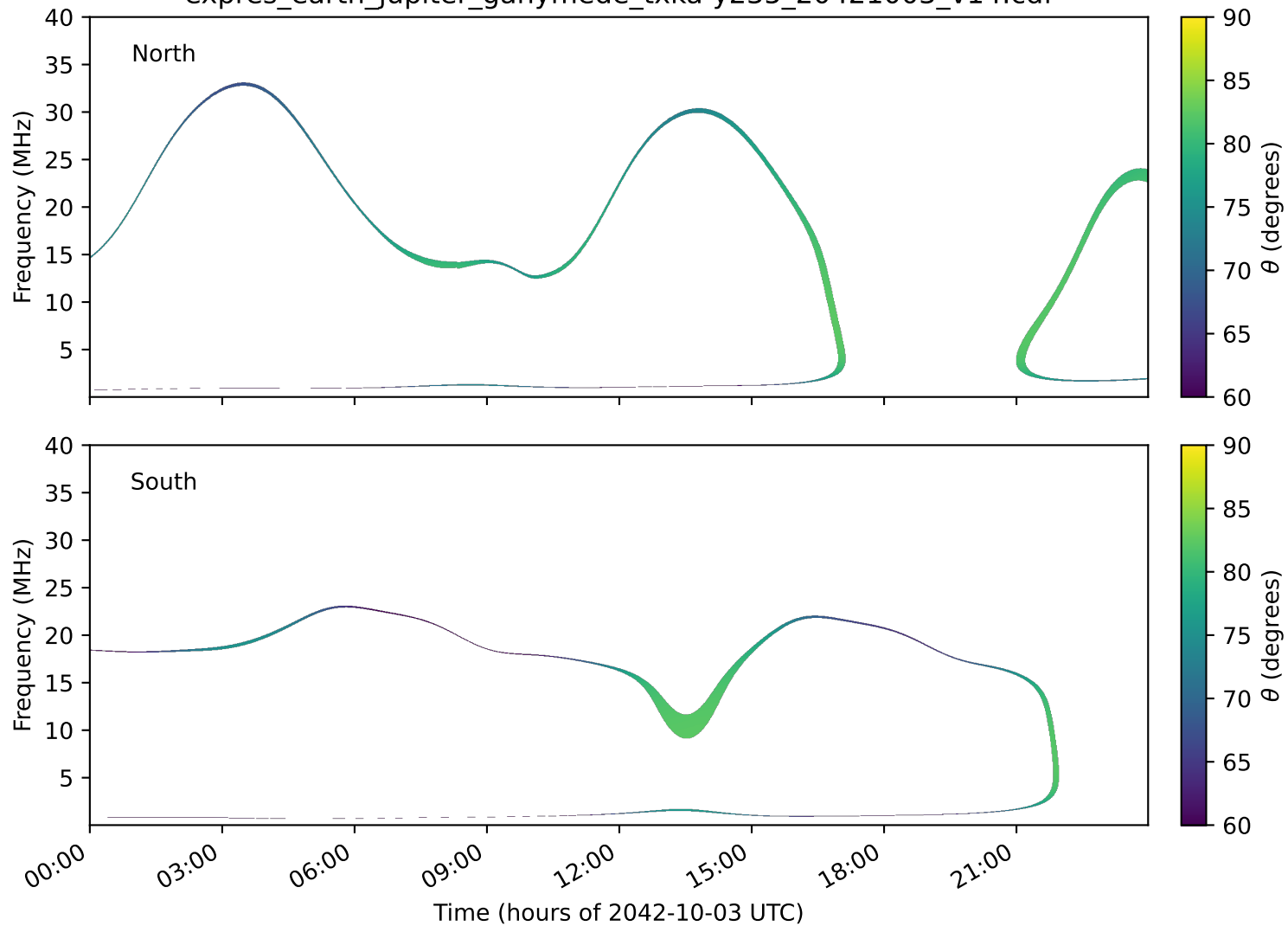
expres_earth_jupiter_ganymede_txka-y235_20421003_v14.cdf
