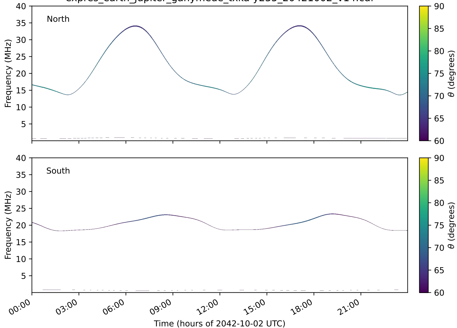
expres_earth_jupiter_ganymede_txka-y235_20421002_v14.cdf
