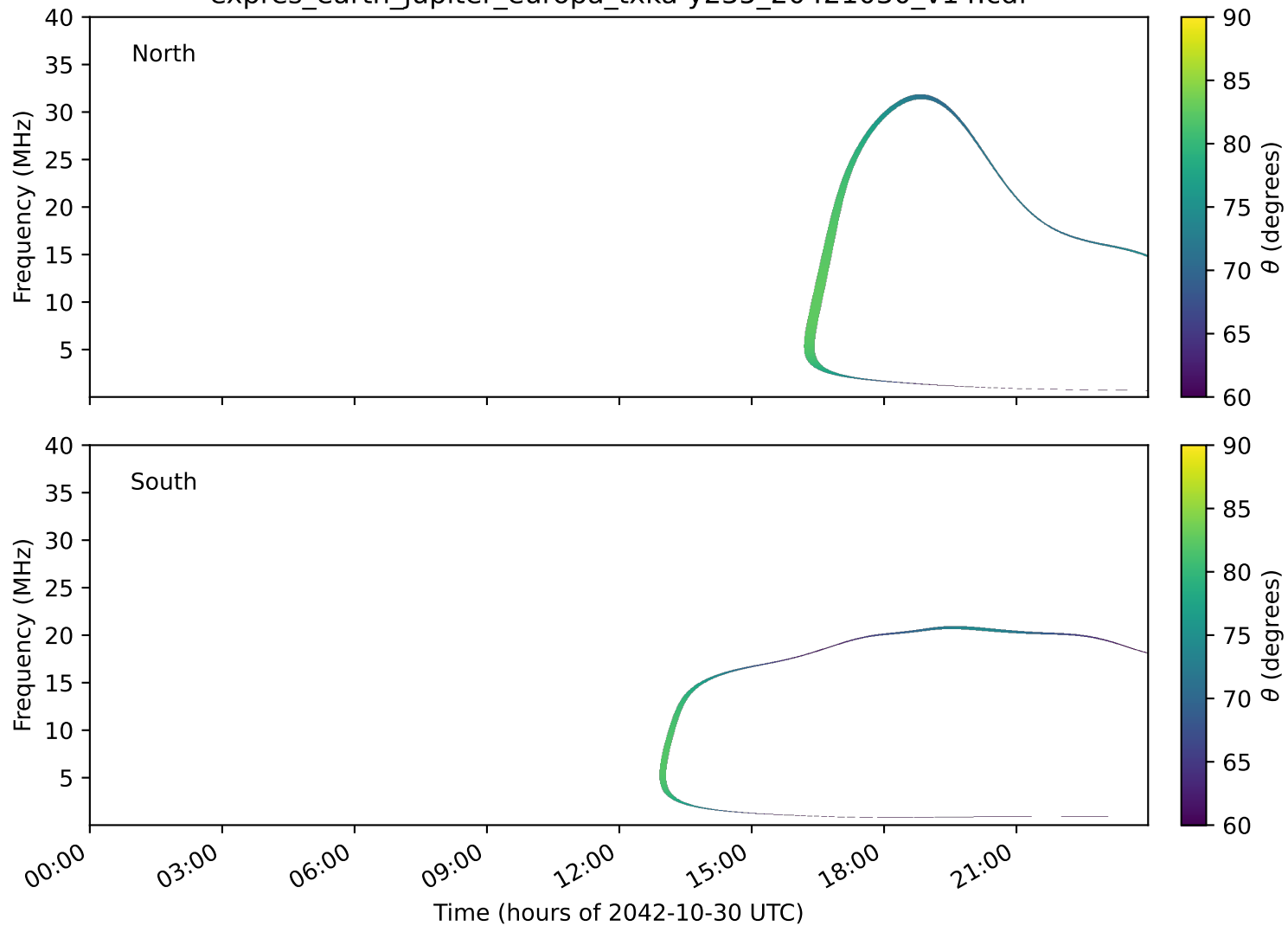
expres_earth_jupiter_europa_txka-y235_20421030_v14.cdf
