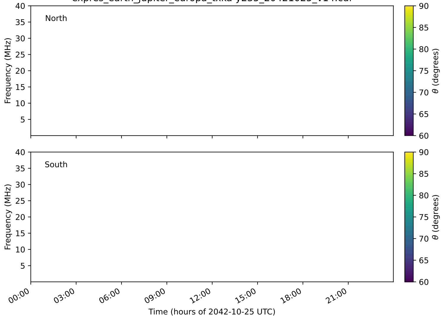
expres_earth_jupiter_europa_txka-y235_20421025_v14.cdf
