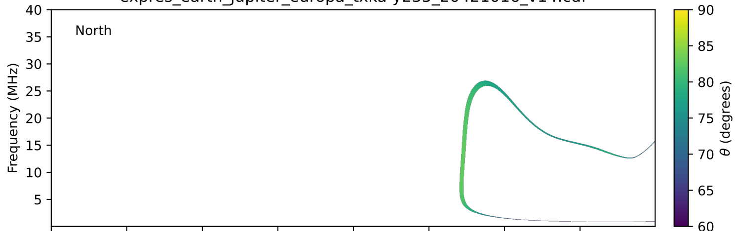
expres_earth_jupiter_europa_txka-y235_20421016_v14.cdf
