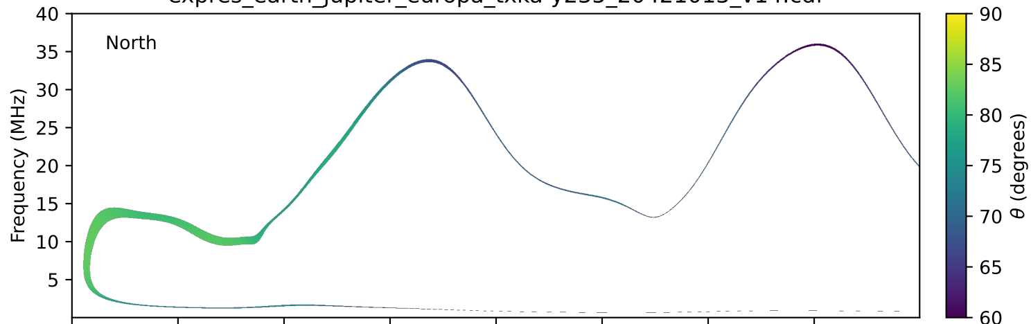
expres_earth_jupiter_europa_txka-y235_20421013_v14.cdf
