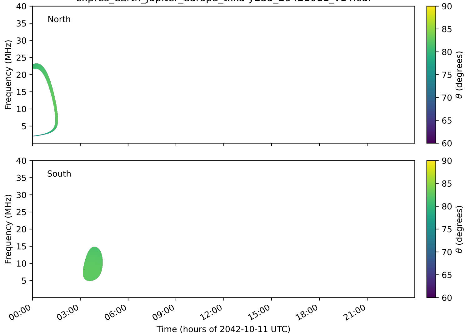
expres_earth_jupiter_europa_txka-y235_20421011_v14.cdf
