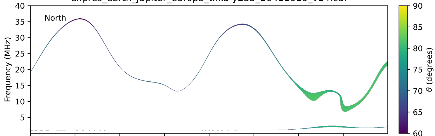
expres_earth_jupiter_europa_txka-y235_20421010_v14.cdf
