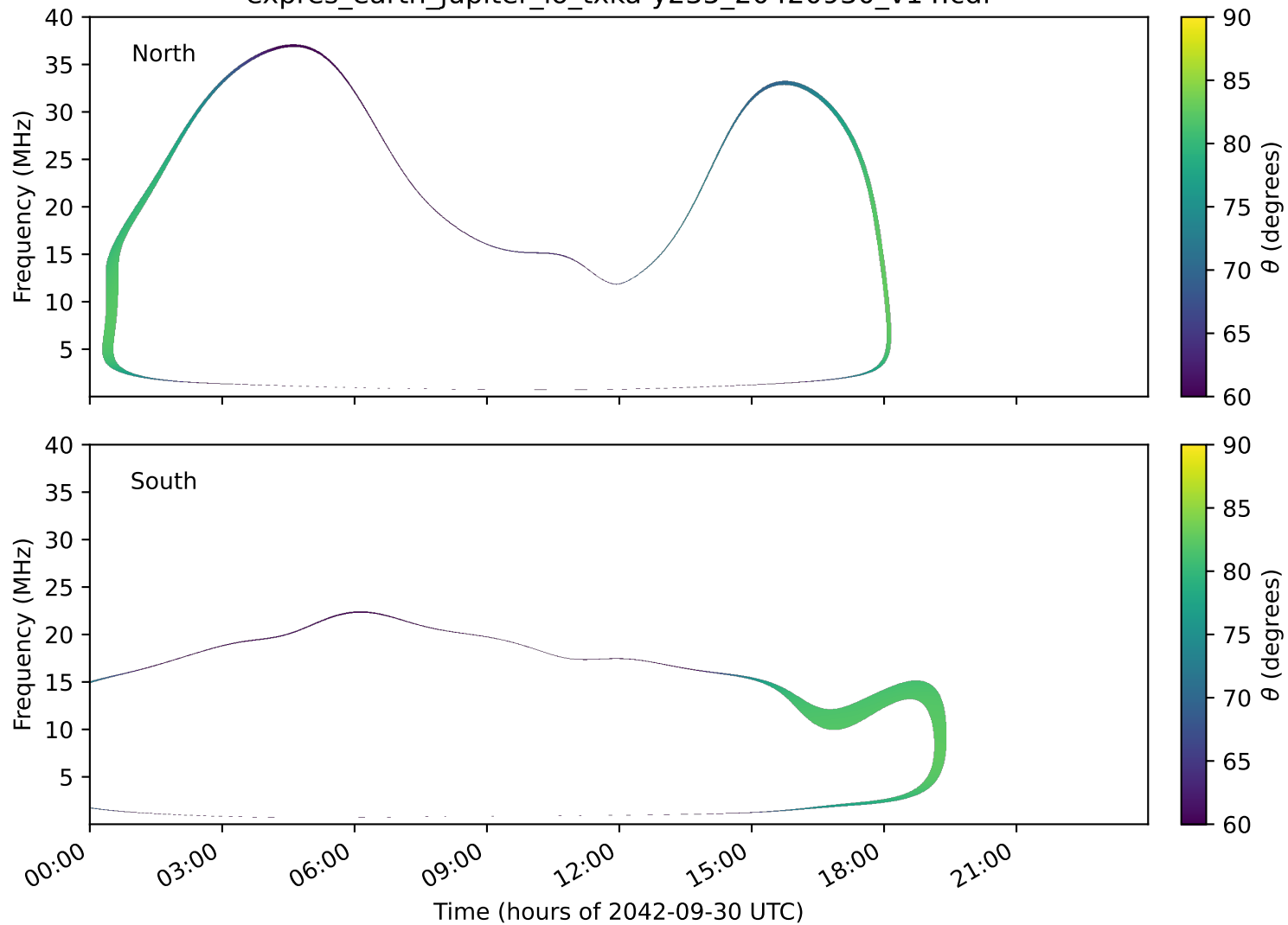
expres_earth_jupiter_io_txka-y235_20420930_v14.cdf
