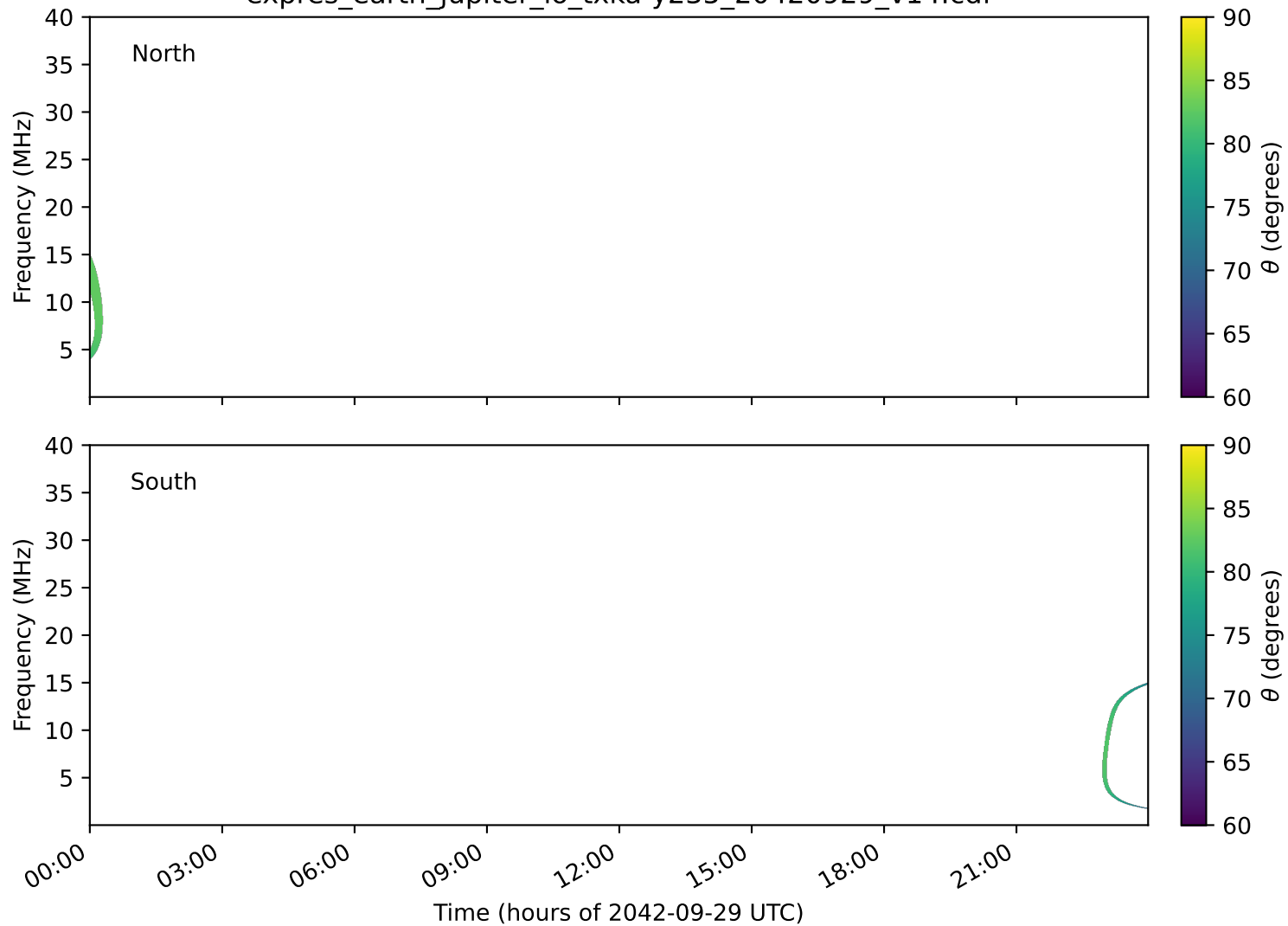
expres_earth_jupiter_io_txka-y235_20420929_v14.cdf
