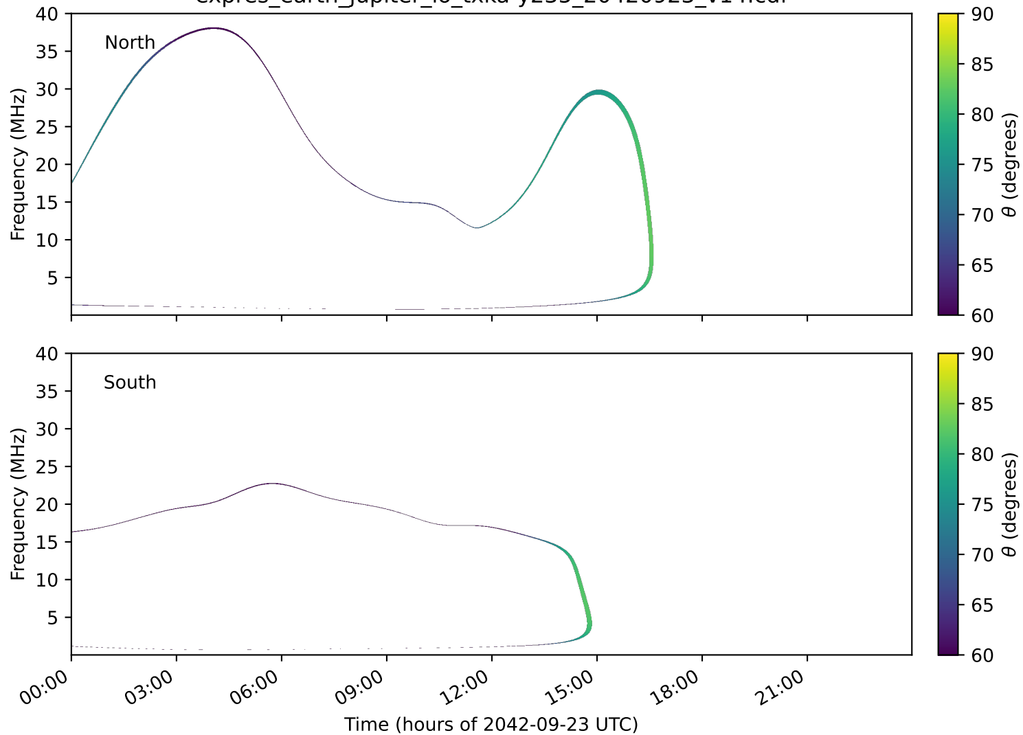
expres_earth_jupiter_io_txka-y235_20420923_v14.cdf
