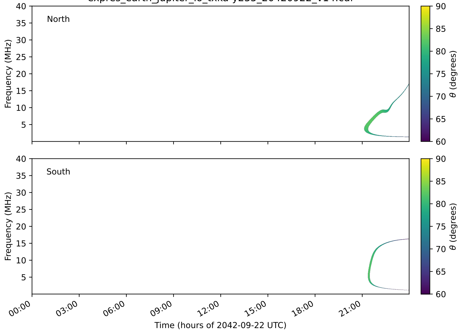
expres_earth_jupiter_io_txka-y235_20420922_v14.cdf
