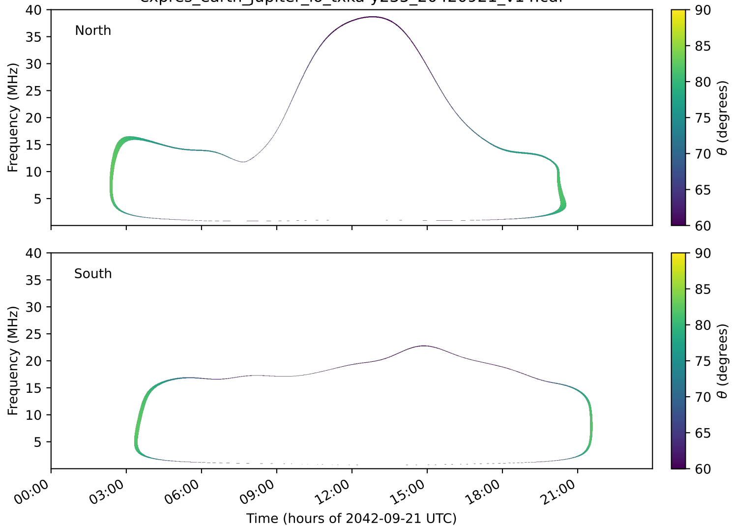
expres_earth_jupiter_io_txka-y235_20420921_v14.cdf
