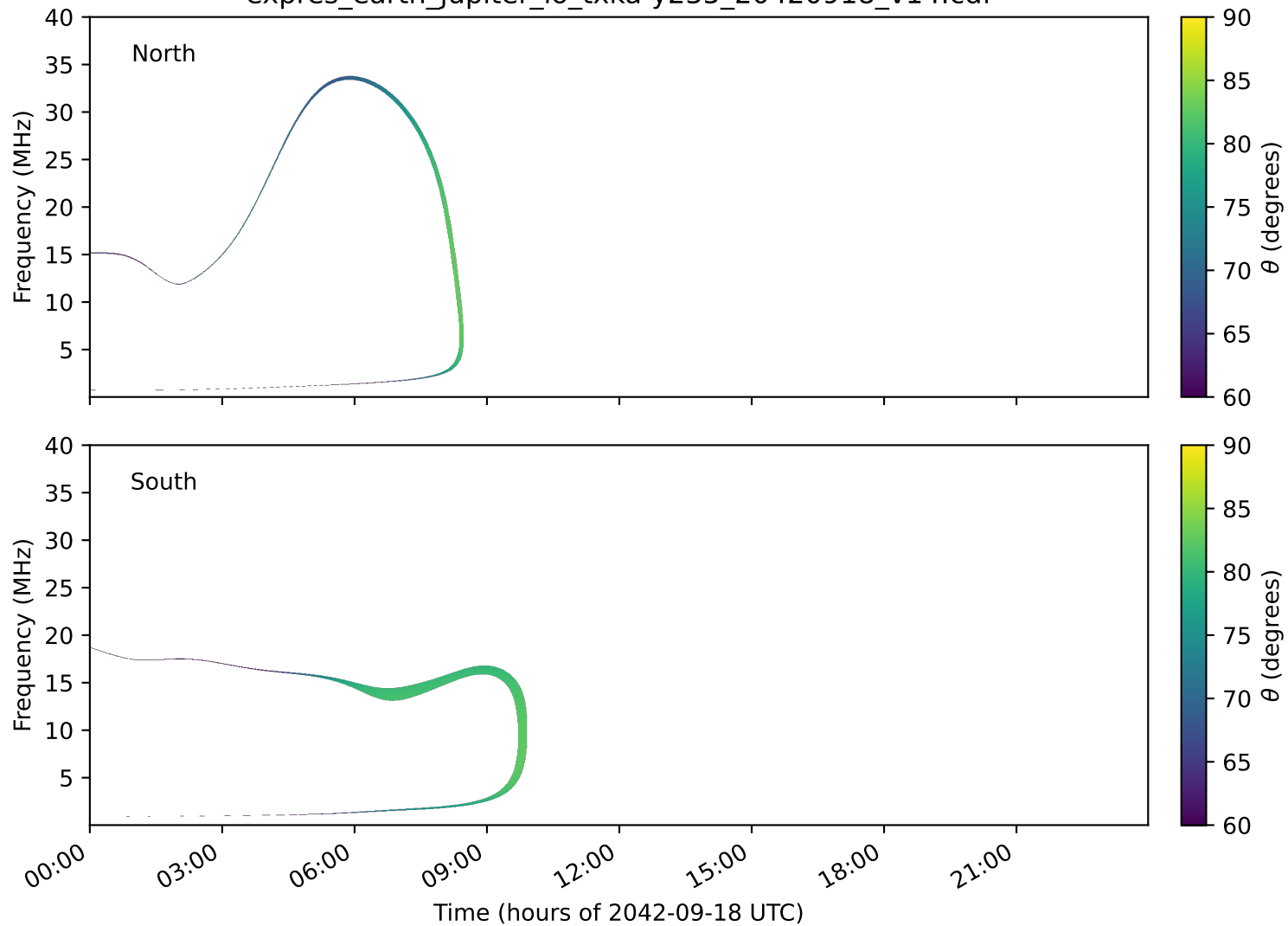
expres_earth_jupiter_io_txka-y235_20420918_v14.cdf
