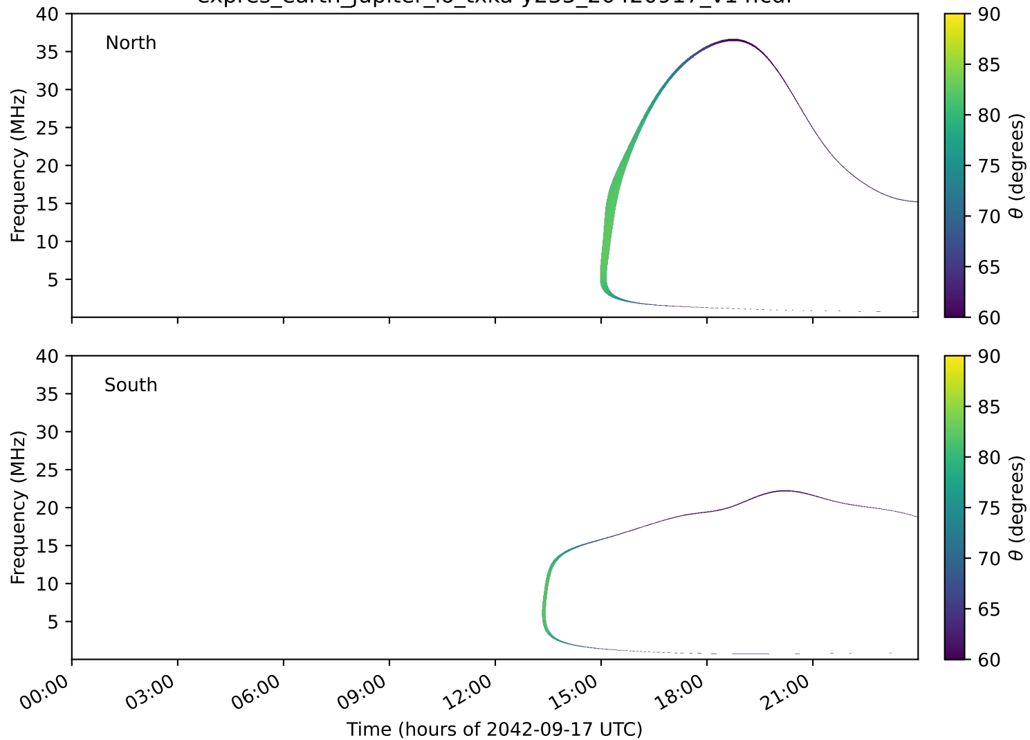
expres_earth_jupiter_io_txka-y235_20420917_v14.cdf
