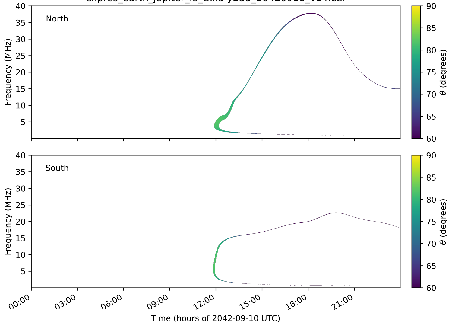
expres_earth_jupiter_io_txka-y235_20420910_v14.cdf
