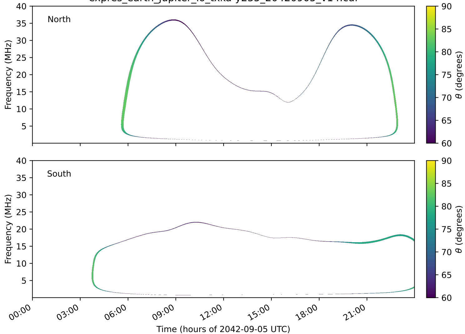
expres_earth_jupiter_io_txka-y235_20420905_v14.cdf
