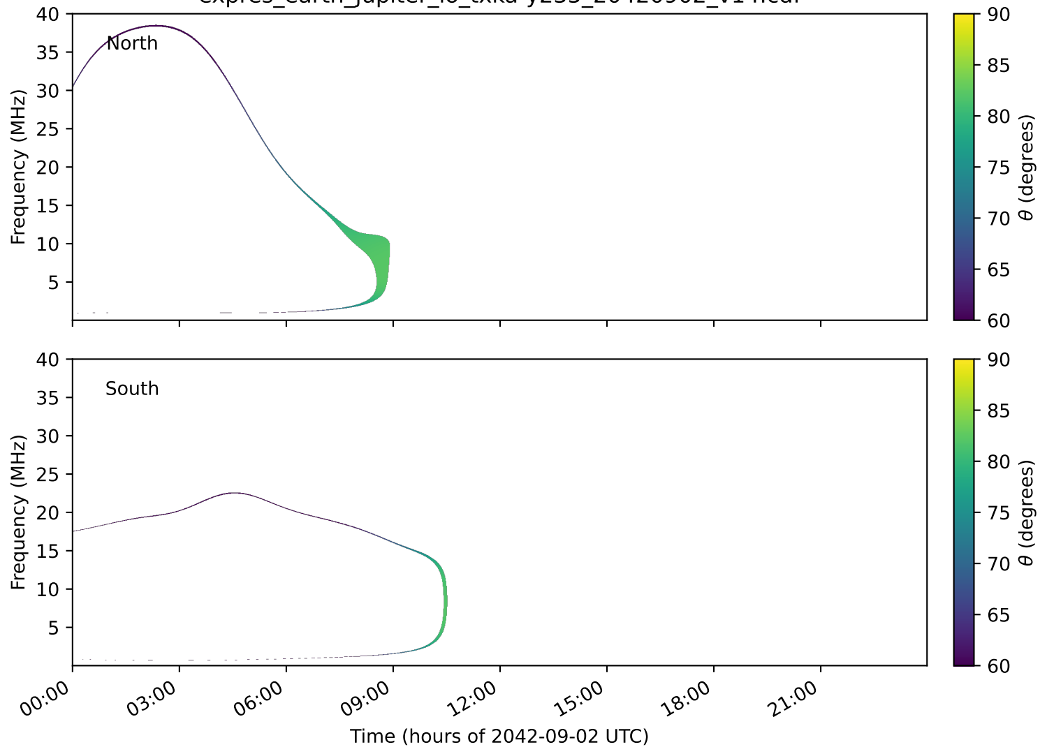
expres_earth_jupiter_io_txka-y235_20420902_v14.cdf
