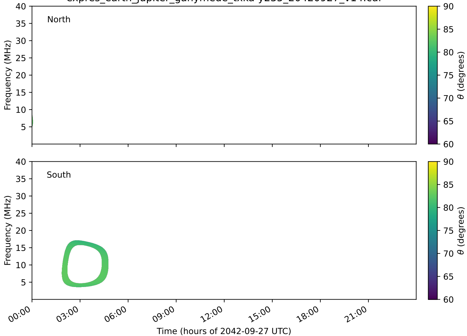
expres_earth_jupiter_ganymede_txka-y235_20420927_v14.cdf
