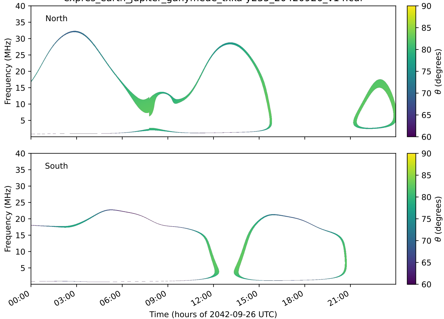
expres_earth_jupiter_ganymede_txka-y235_20420926_v14.cdf
