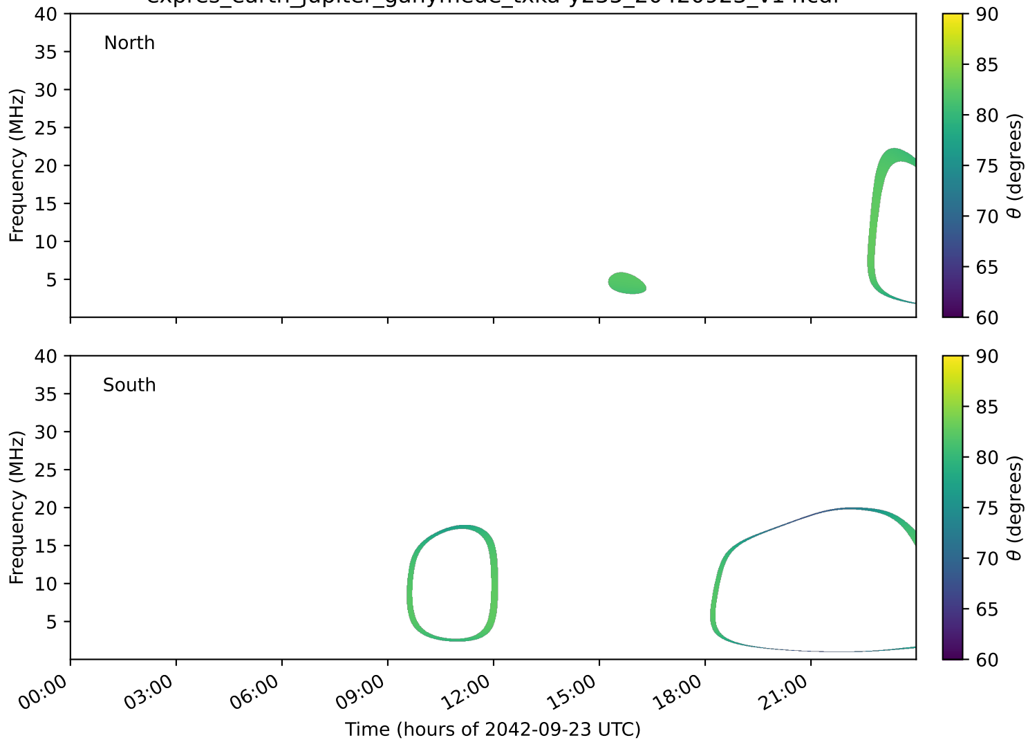
expres_earth_jupiter_ganymede_txka-y235_20420923_v14.cdf
