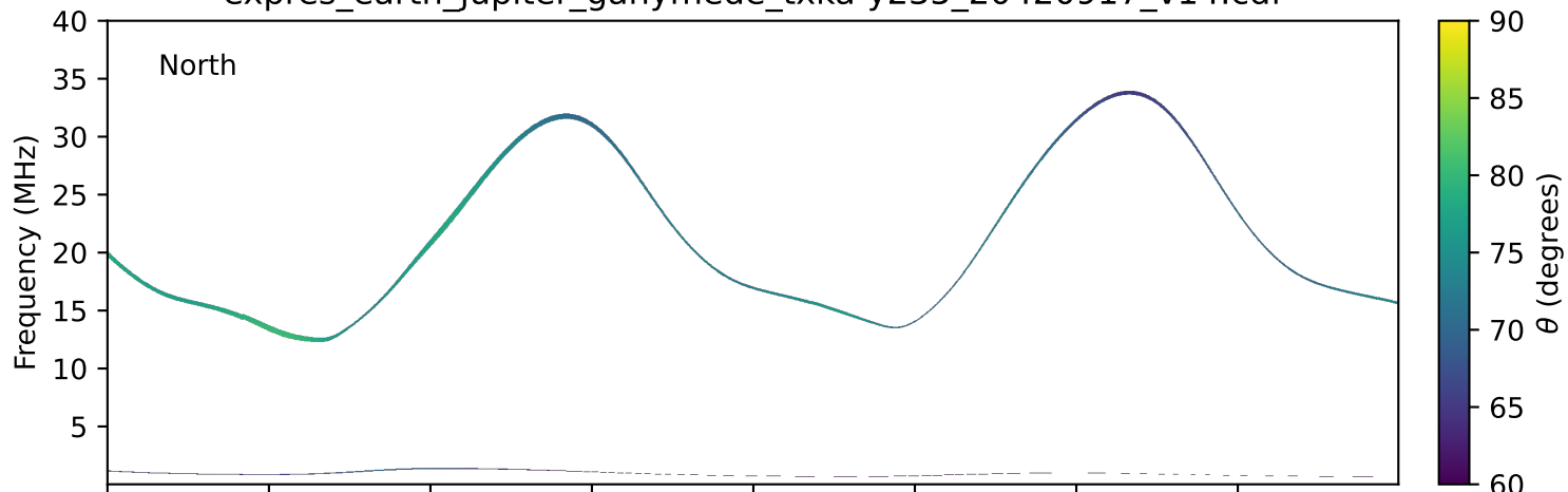
expres_earth_jupiter_ganymede_txka-y235_20420917_v14.cdf
