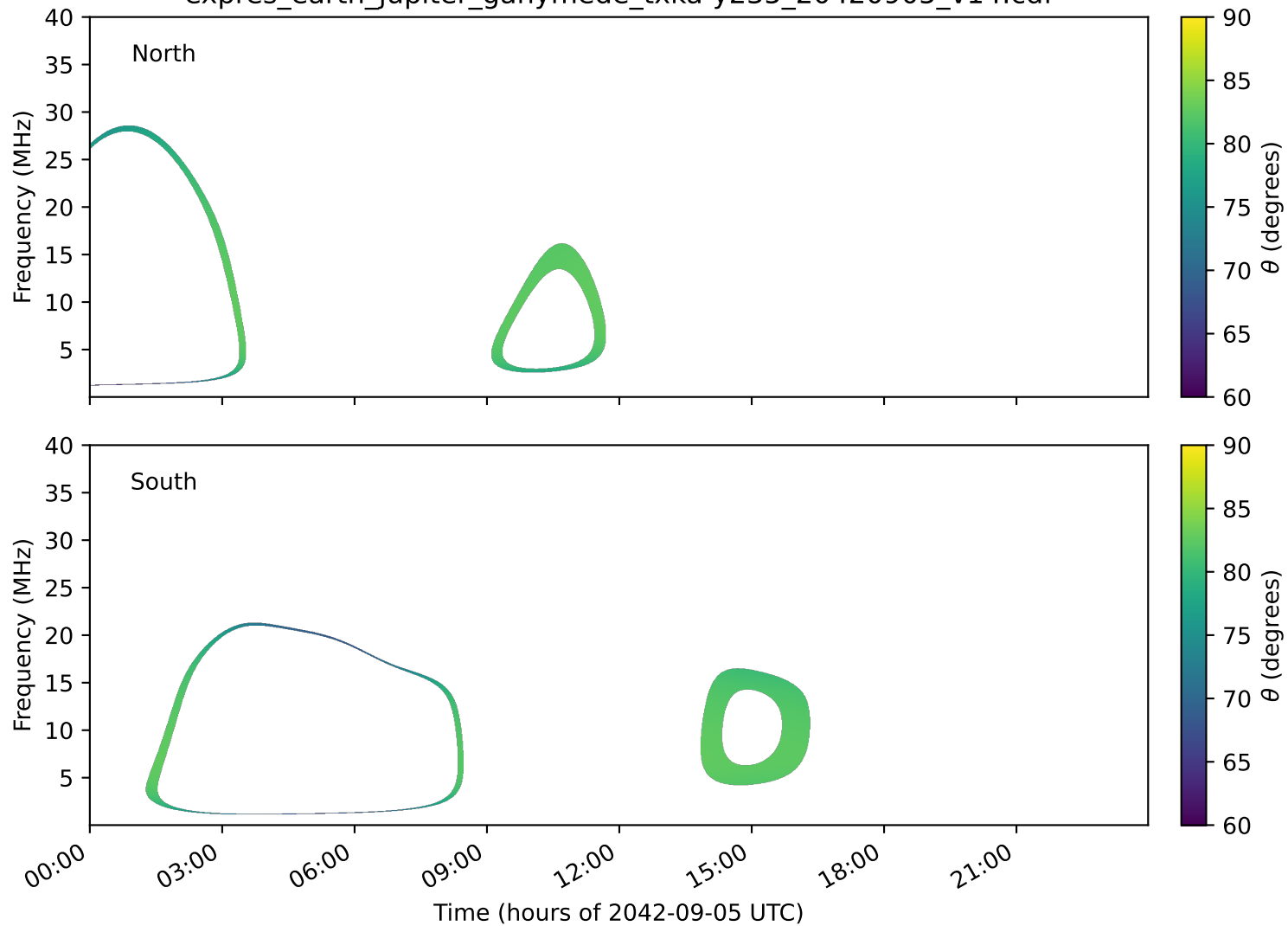
expres_earth_jupiter_ganymede_txka-y235_20420905_v14.cdf
