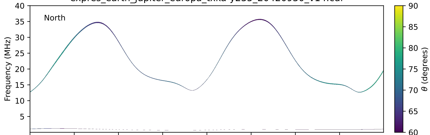
expres_earth_jupiter_europa_txka-y235_20420930_v14.cdf
