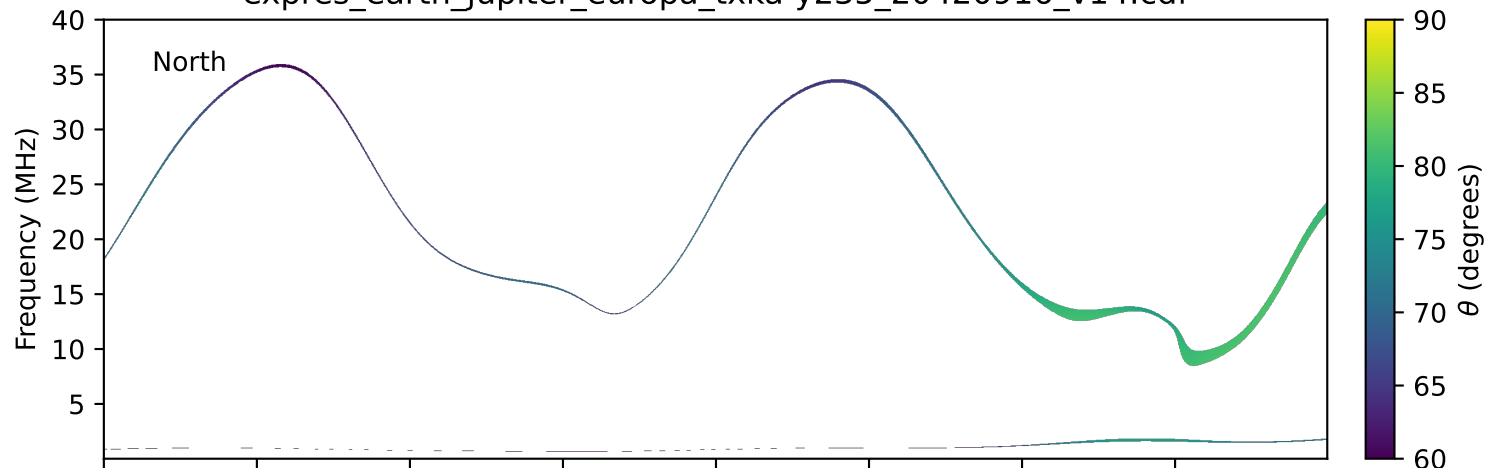
expres_earth_jupiter_europa_txka-y235_20420916_v14.cdf
