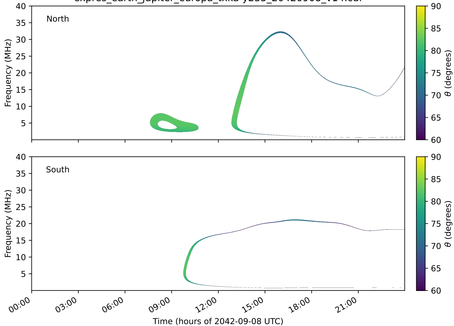
expres_earth_jupiter_europa_txka-y235_20420908_v14.cdf
