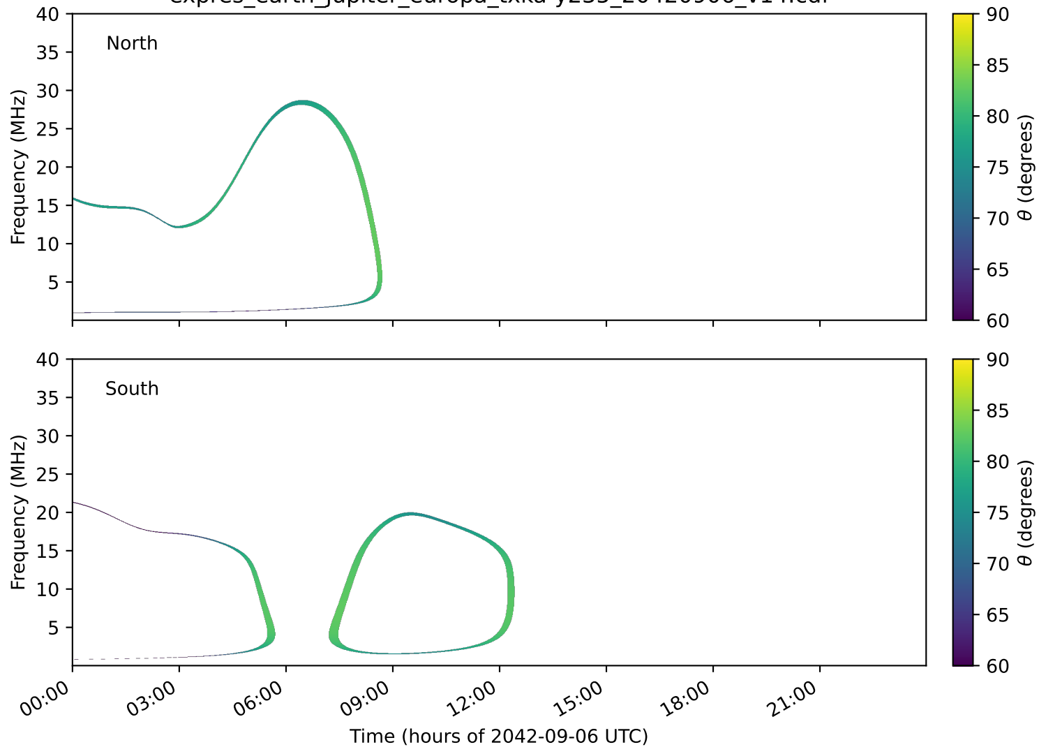
expres_earth_jupiter_europa_txka-y235_20420906_v14.cdf
