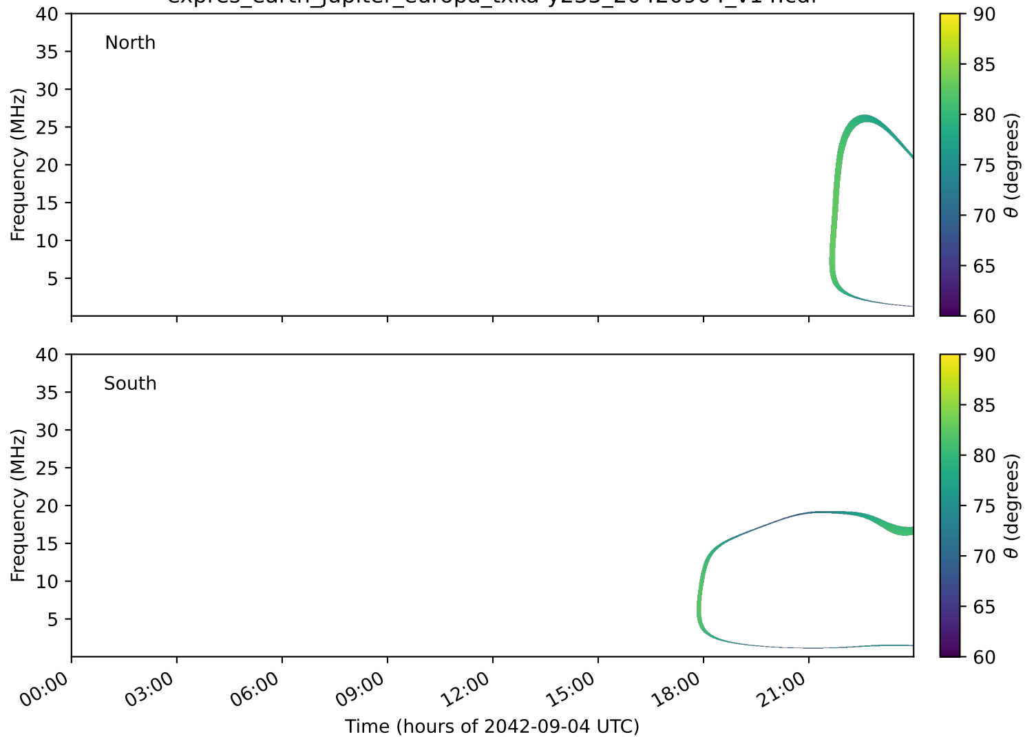
expres_earth_jupiter_europa_txka-y235_20420904_v14.cdf
