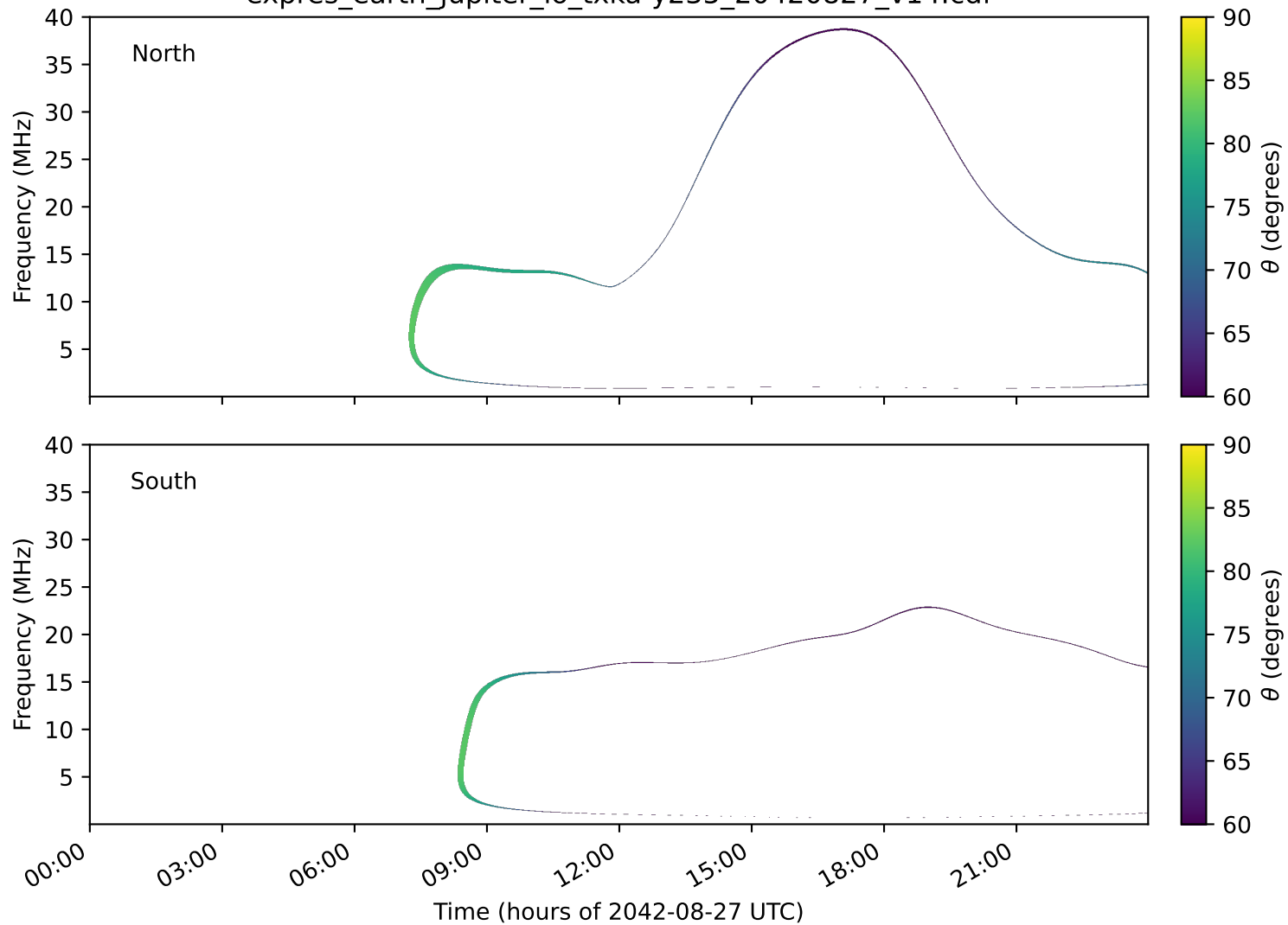
expres_earth_jupiter_io_txka-y235_20420827_v14.cdf
