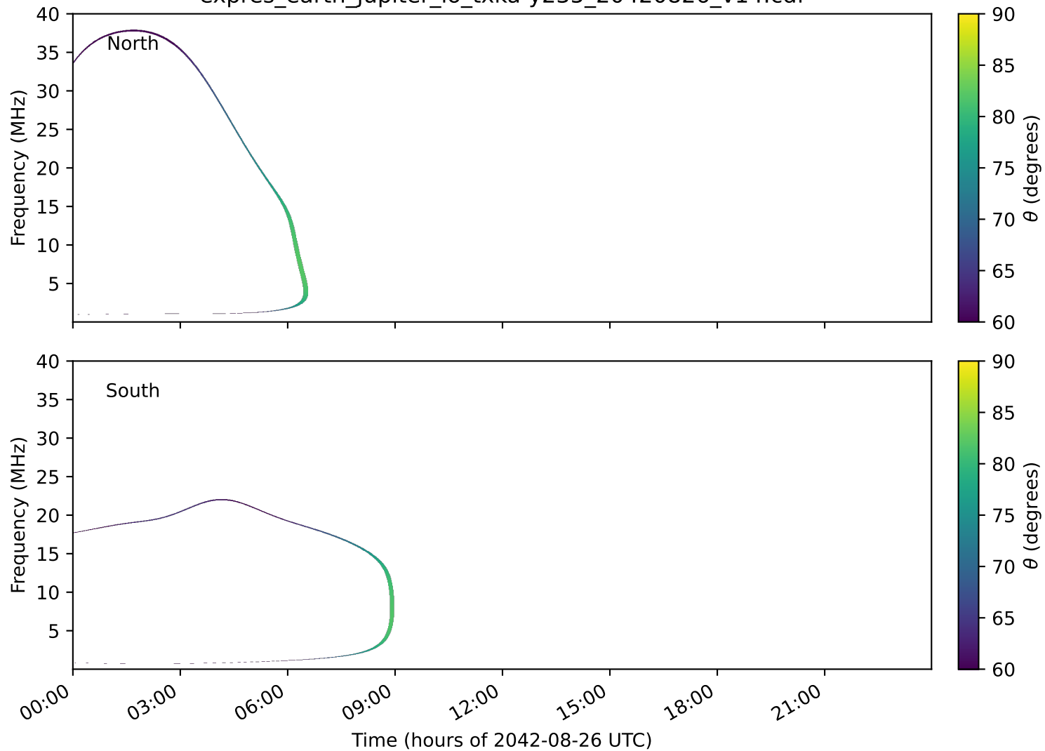
expres_earth_jupiter_io_txka-y235_20420826_v14.cdf
